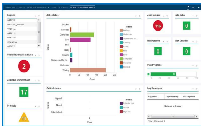
Dashboard
